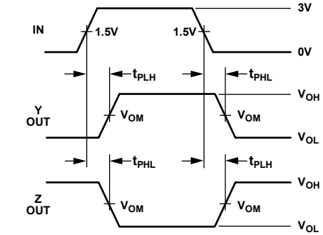
Figure 11. Driver Propagation Delays
