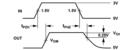
Figure 14. Driver Enable and Disable Times ( t_{PZH} , t_{PSH} , t_{PHZ} )
